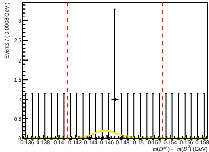
Passed ( 200 < nTracks < 600 , 3.6 < \eta < 5.0 , 27000 < p < 60000 )
