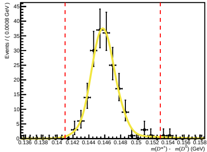
Failed ( 200 < nTracks < 600 , 3.6 < \eta < 5.0 , 27000 < p < 60000 )
