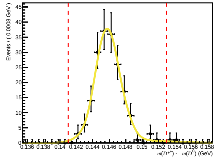
Total ( 200 < nTracks < 600 , 3.6 < \eta < 5.0 , 27000 < p < 60000 )
