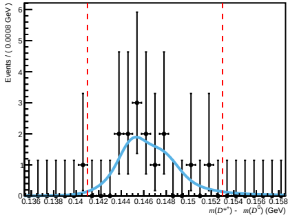
Passed ( 0 < n_{\text{Tracks}} < 200 , 1.7 < \eta < 3.6 , 6000 < p < 10000 )
