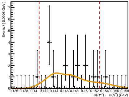
Passed ( 0 < nTracks < 200 , 1.7 < \eta < 3.6 , 60000 < p < 100000 )
