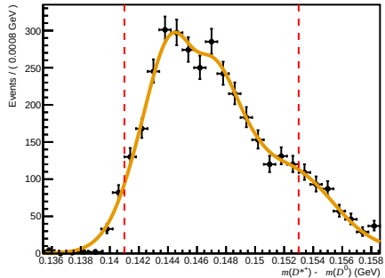
Failed ( 0 < nTracks < 200 , 1.7 < \eta < 3.6 , 60000 < p < 100000 )
