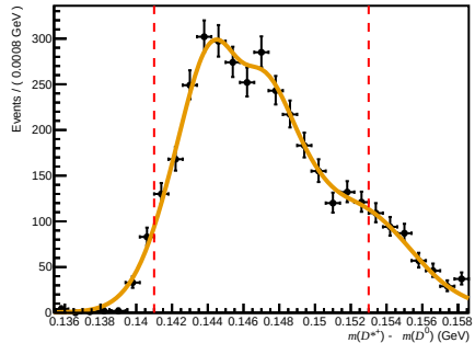
Total ( 0 < nTracks < 200 , 1.7 < \eta < 3.6 , 60000 < p < 100000 )
