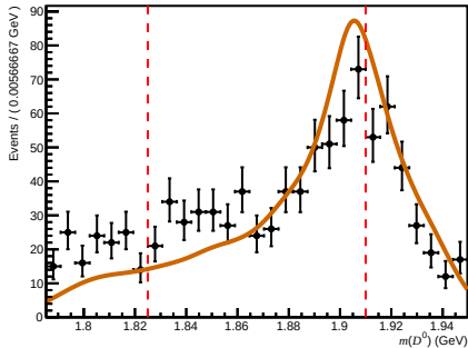
Passed ( 0 < nTracks < 200 , 3.6 < \eta < 5.0 , 10000 < p < 15600 )
