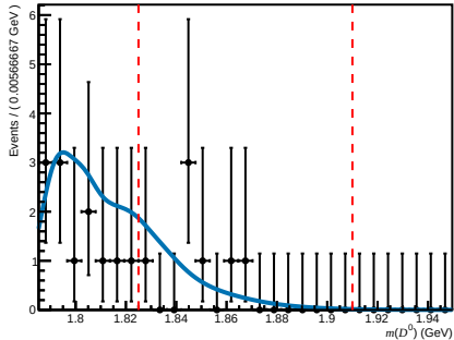
Failed ( 200 < nTracks < 600 , 1.7 < \eta < 3.6 , 3000 < p < 6000 )
