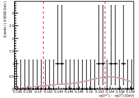
Total ( 200 < nTracks < 600 , 1.7 < \eta < 3.6 , 10000 < p < 15600 )
