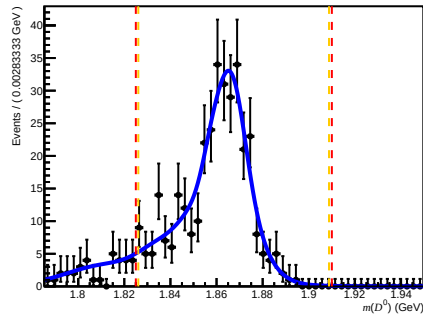
Failed DiF ( 200 < nTracks < 600 , 1.7 < \eta < 3.6 , 15600 < p < 27000 )
