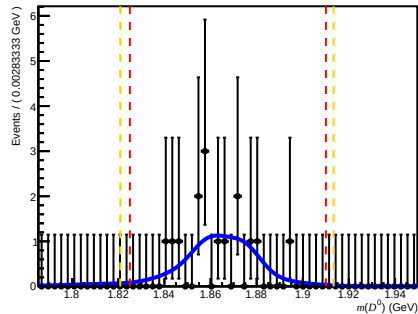
Failed DiF ( 200 < nTracks < 600 , 3.6 < \eta < 5.0 , 3000 < p < 6000 )
