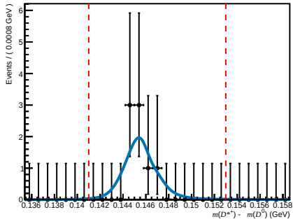
Failed ( 200 < nTracks < 600 , 3.6 < \eta < 5.0 , 6000 < p < 10000 )
