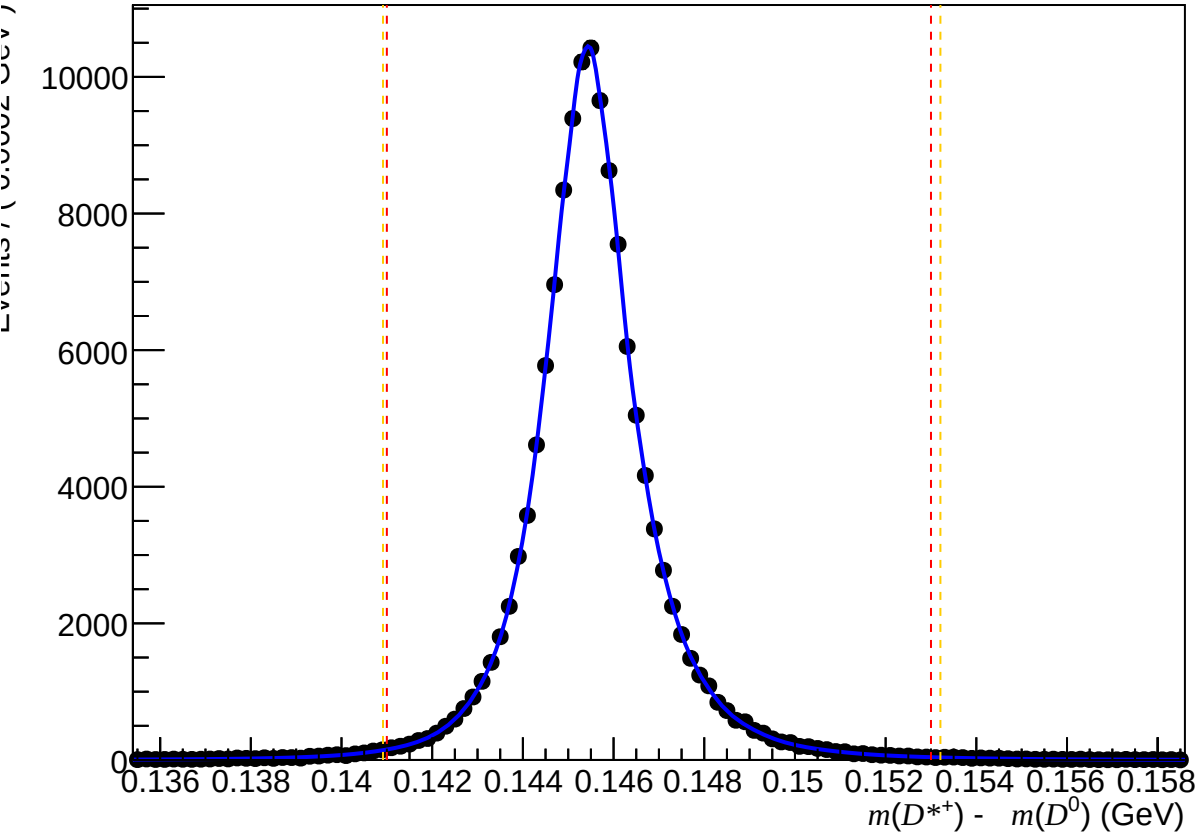
Failed non-DiF ( 200 < n\text{Tracks} < 600 , 3.6 < \eta < 5.0 , 6000 < p < 10000 )
