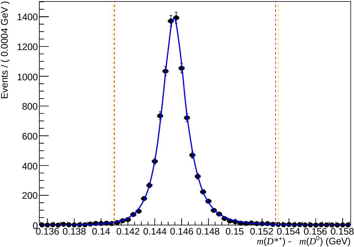
Passed non-DiF ( 200 < n\text{Tracks} < 600 , 3.6 < \eta < 5.0 , 6000 < p < 10000 )
