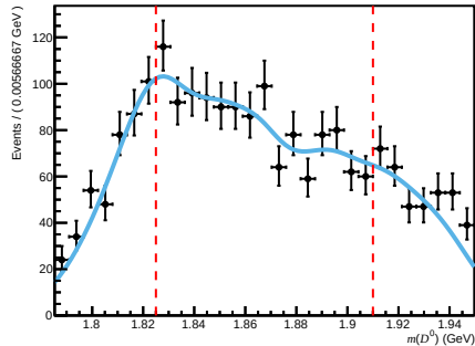
Total ( 200 < n\text{Tracks} < 600 , 3.6 < \eta < 5.0 , 27000 < p < 60000 )
