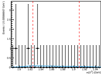
Passed ( 200 < n\text{Tracks} < 600 , 3.6 < \eta < 5.0 , 27000 < p < 60000 )
