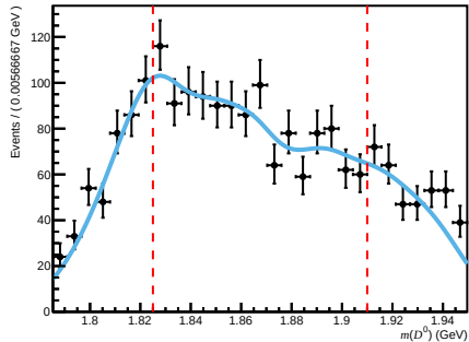
Failed ( 200 < n\text{Tracks} < 600 , 3.6 < \eta < 5.0 , 27000 < p < 60000 )
