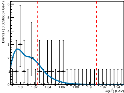
Passed ( 0 < n\text{Tracks} < 200 , 1.7 < \eta < 3.6 , 15600 < p < 27000 )
