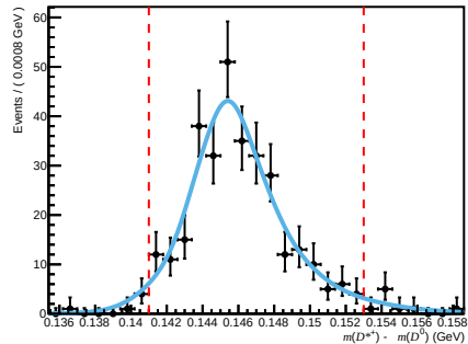
Total ( 0 < n_{\text{Tracks}} < 200 , 1.7 < \eta < 3.6 , 60000 < p < 100000 )
