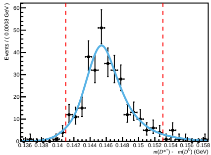
Failed ( 0 < n_{\text{Tracks}} < 200 , 1.7 < \eta < 3.6 , 60000 < p < 100000 )
