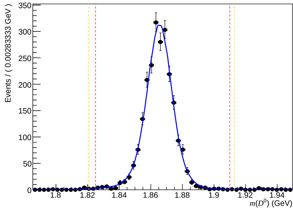
Passed non-DiF ( 0 < nTracks < 200 , 3.6 < \eta < 5.0 , 6000 < p < 10000 )
