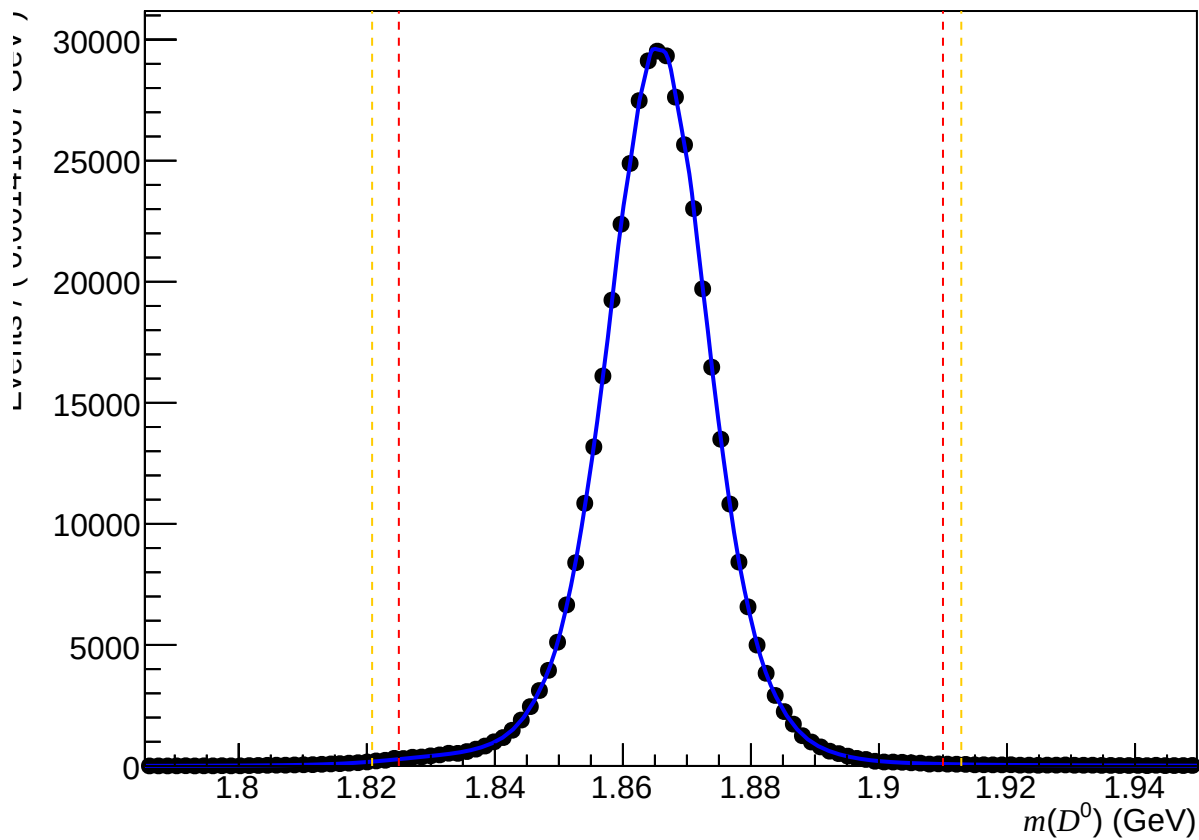
Failed non-DiF ( 0 < nTracks < 200 , 3.6 < \eta < 5.0 , 6000 < p < 10000 )
