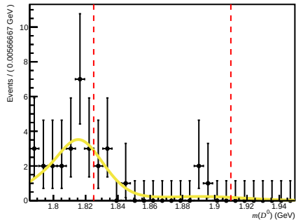
Failed ( 200 < nTracks < 600 , 1.7 < \eta < 3.6 , 10000 < p < 15600 )
