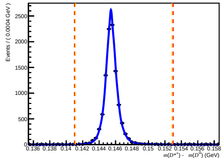
Passed DiF (after RICH1) ( 200 < nTracks < 600 , 1.7 < \eta < 3.6 , 10000 < p < 15600 )
