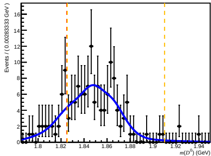
Passed DfF (after RICH1) ( 0 < nTracks < 200 , 1.7 < \eta < 3.6 , 60000 < p < 100000 )
