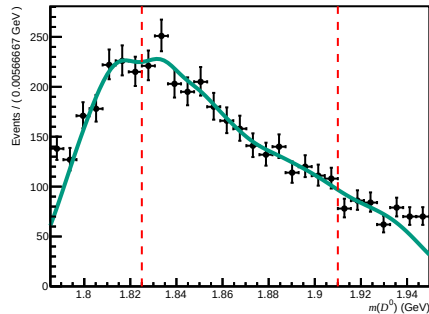
Total ( 0 < nTracks < 200 , 3.6 < \eta < 5.0 , 15600 < p < 27000 )
