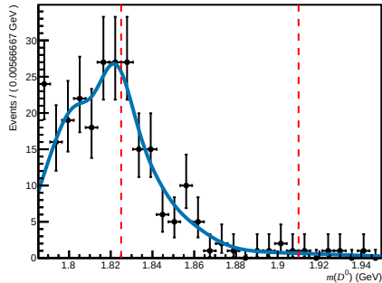
Total ( 200 < nTracks < 600 , 3.6 < \eta < 5.0 , 60000 < p < 100000 )
