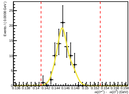
Total ( 0 < nTracks < 200 , 1.7 < \eta < 3.6 , 15600 < p < 27000 )
