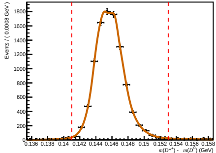
Failed ( 0 < nTracks < 200 , 3.6 < \eta < 5.0 , 60000 < p < 100000 )
