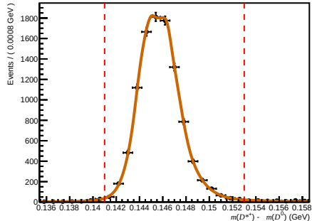
Total ( 0 < nTracks < 200 , 3.6 < \eta < 5.0 , 60000 < p < 100000 )
