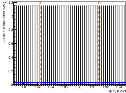
Passed DfF (before RICH1) ( 200 < nTracks < 600 , 1.7 < \eta < 3.6 , 6000 < p < 10000 )
