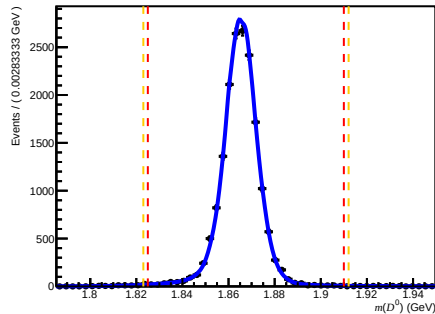
Failed DfF ( 200 < nTracks < 600 , 1.7 < \eta < 3.6 , 6000 < p < 10000 )
