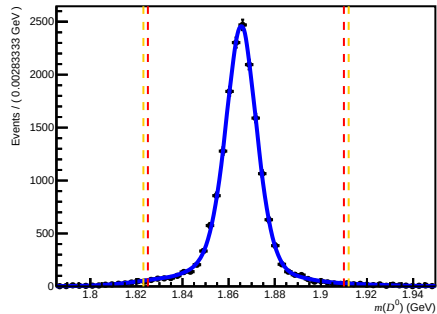
Passed DfF (after RICH1) ( 200 < nTracks < 600 , 1.7 < \eta < 3.6 , 6000 < p < 10000 )
