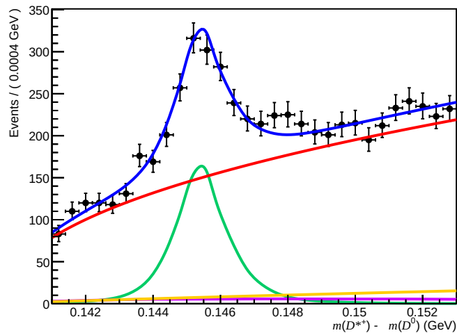
Passed ( 200 < n\text{Tracks} < 600 , 3.6 < \eta < 5.0 , 3000 < p < 6000 )
