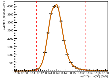
Failed ( 200 < nTracks < 600 , 3.6 < \eta < 5.0 , 27000 < p < 60000 )
