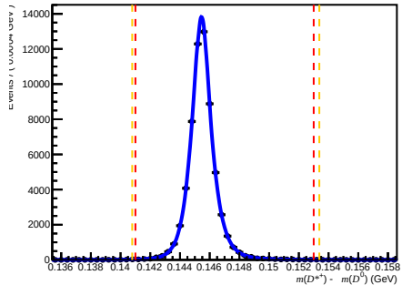
Passed DiF (after RICH1) ( 0 < nTracks < 200 , 1.7 < \eta < 3.6 , 3000 < p < 6000 )
