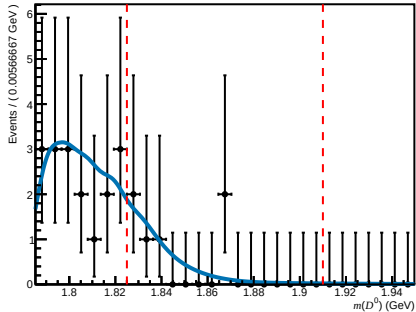
Failed ( 0 < nTracks < 200 , 1.7 < \eta < 3.6 , 15600 < p < 27000 )
