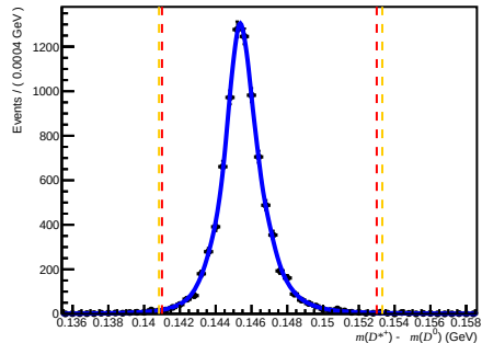
Passed DIF (after RICH1) ( 0 < nTracks < 200 , 3.6 < \eta < 5.0 , 6000 < p < 10000 )
