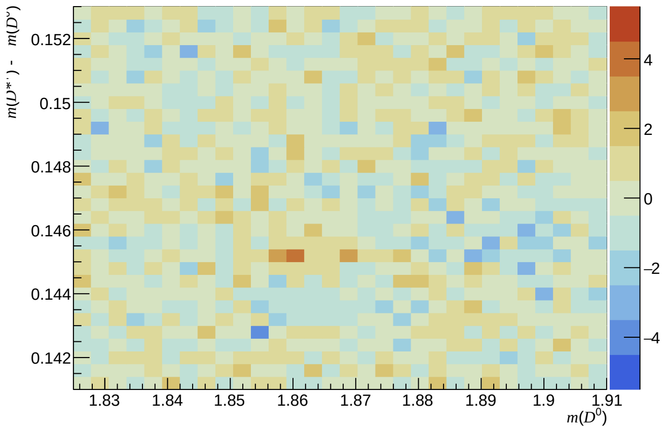
Passed ( 0 < nTracks < 200 , 3.6 < \eta < 5.0 , 10000 < p < 15600 )
