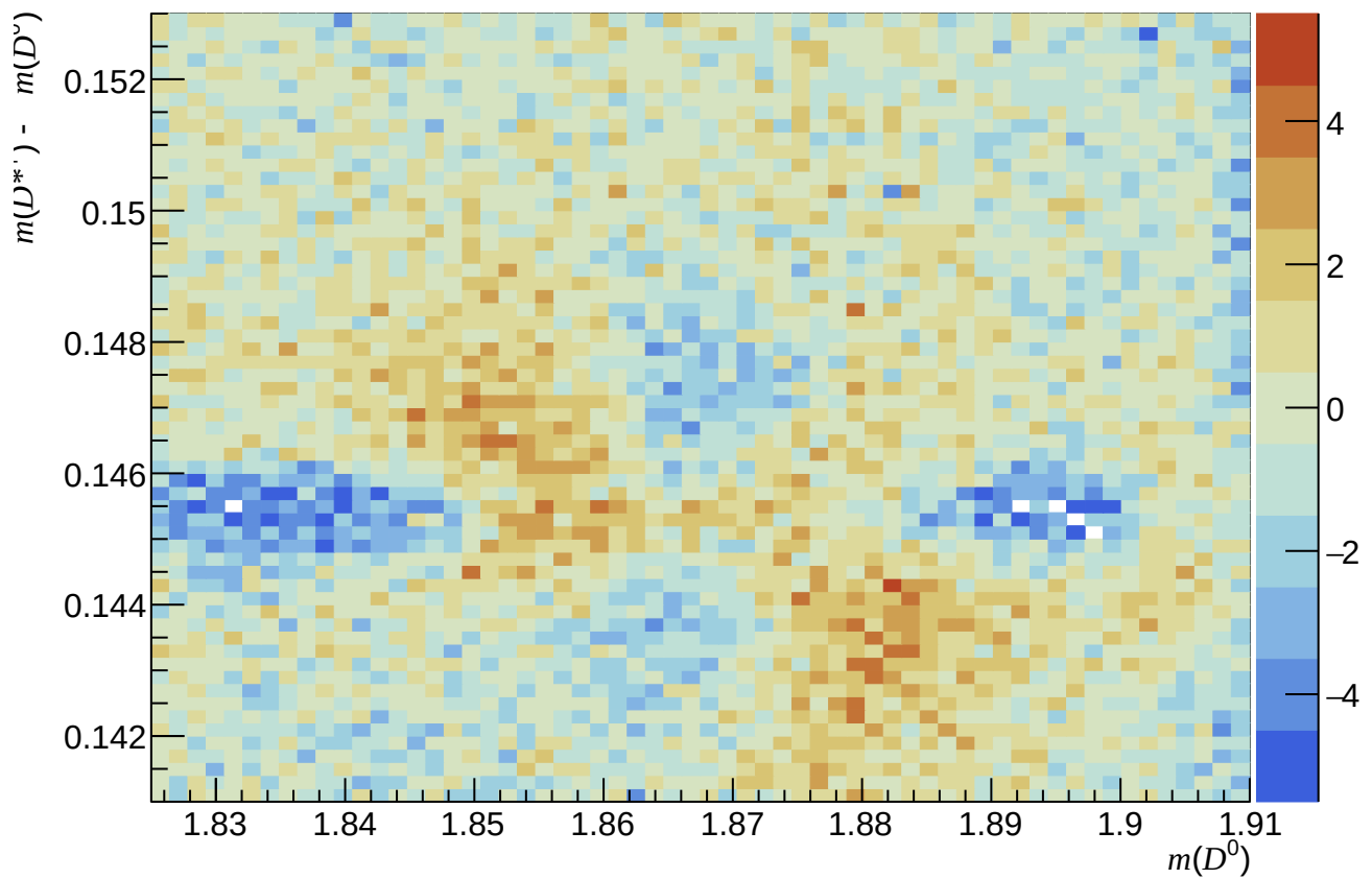
Failed ( 0 < nTracks < 200 , 3.6 < \eta < 5.0 , 10000 < p < 15600 )
