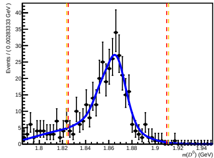
Failed DiF ( 0 < n_{\text{Tracks}} < 200 , 3.6 < \eta < 5.0 , 15600 < p < 27000 )
