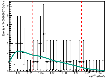
Failed ( 200 < nTracks < 600 , 1.7 < \eta < 3.6 , 10000 < p < 15600 )
