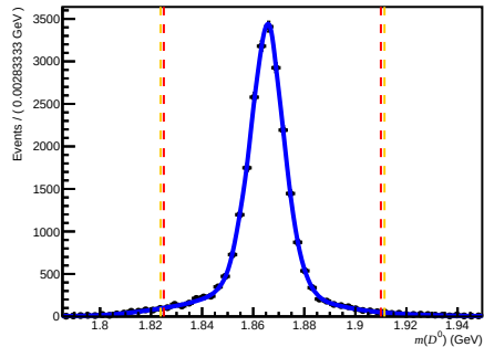
Passed DfF (after RICH1) ( 0 < nTracks < 200 , 1.7 < \eta < 3.6 , 6000 < p < 10000 )
