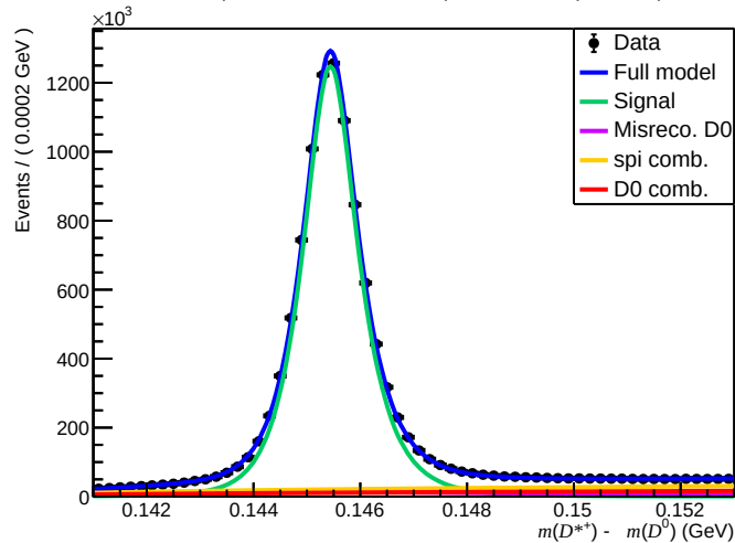
Failed ( 0 < n_{\text{Tracks}} < 200 , 1.7 < \eta < 3.6 , 10000 < p < 15600 )
