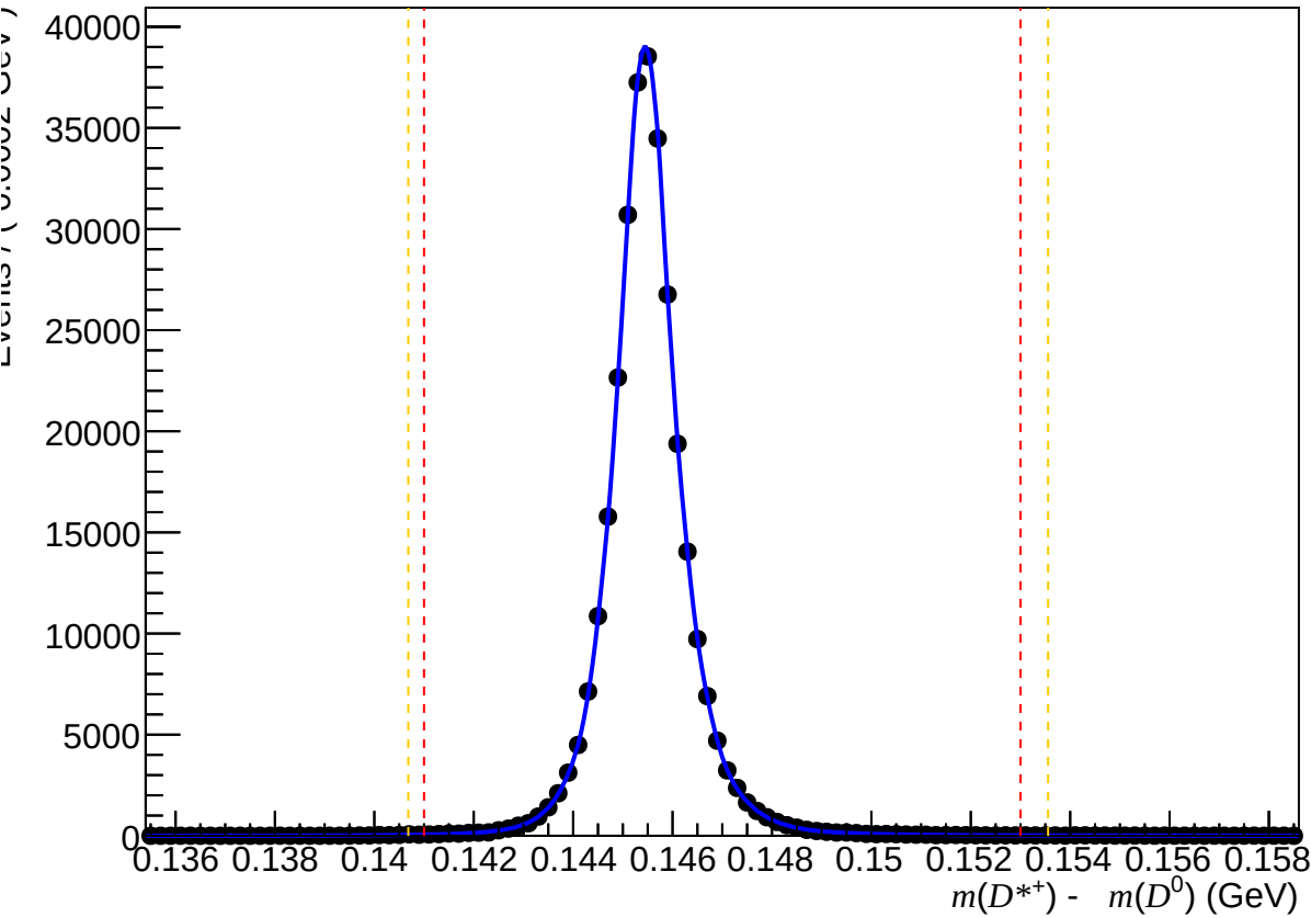
Failed non-DiF ( 200 < nTracks < 600 , 1.7 < \eta < 3.6 , 3000 < p < 6000 )
