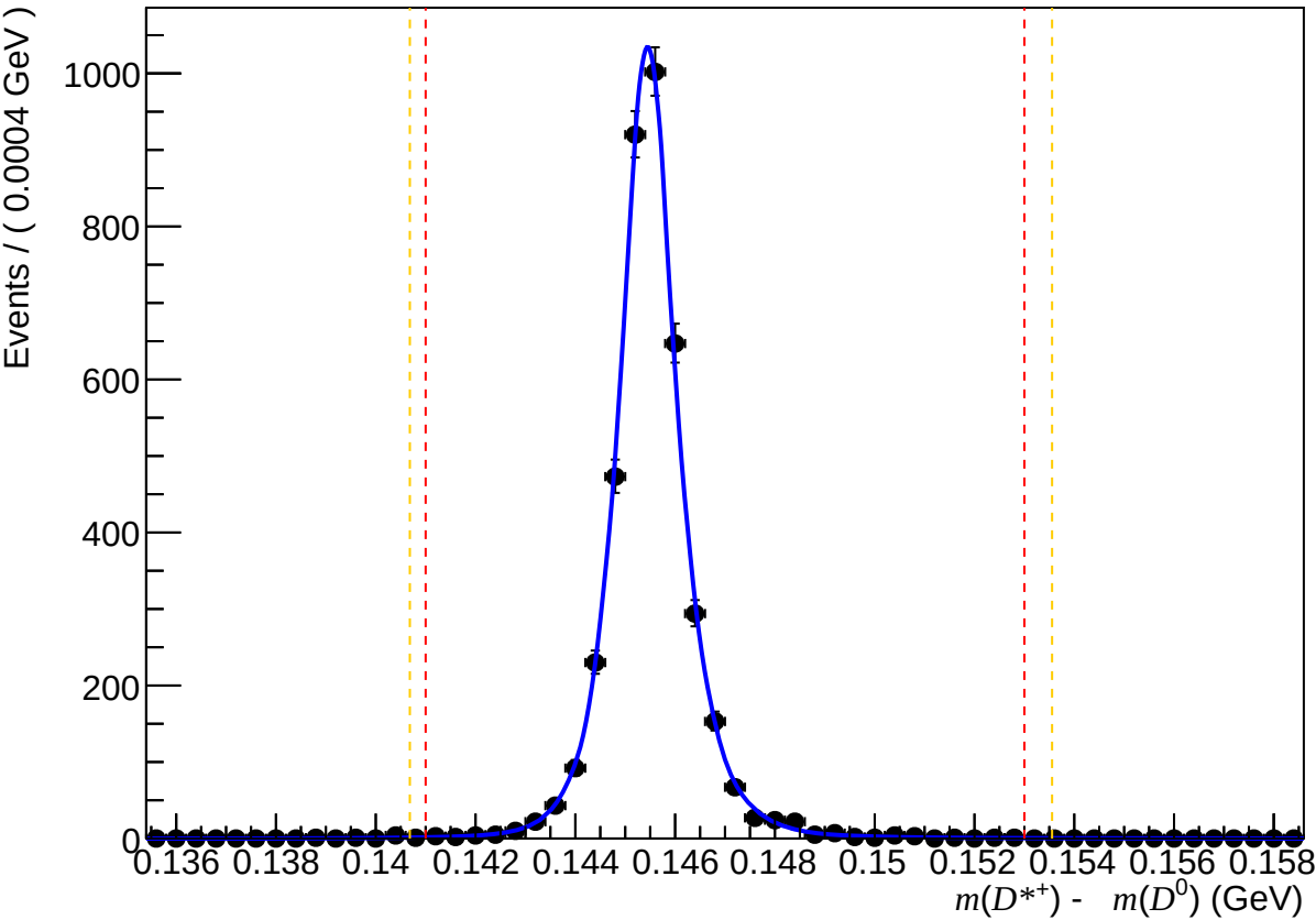
Passed non-DiF ( 200 < nTracks < 600 , 1.7 < \eta < 3.6 , 3000 < p < 6000 )
