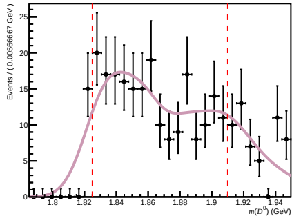
Failed ( 200 < nTracks < 600 , 1.7 < \eta < 3.6 , 10000 < p < 15600 )
