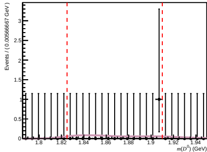
Passed ( 200 < nTracks < 600 , 1.7 < \eta < 3.6 , 10000 < p < 15600 )
