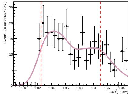
Total ( 200 < nTracks < 600 , 1.7 < \eta < 3.6 , 10000 < p < 15600 )
