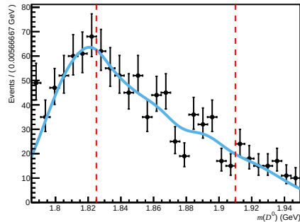
Total ( 200 < nTracks < 600 , 1.7 < \eta < 3.6 , 15600 < p < 27000 )
