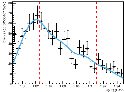
Failed ( 200 < nTracks < 600 , 1.7 < \eta < 3.6 , 15600 < p < 27000 )
