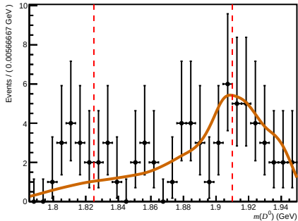
Passed ( 0 < nTracks < 200 , 1.7 < \eta < 3.6 , 15600 < p < 27000 )
