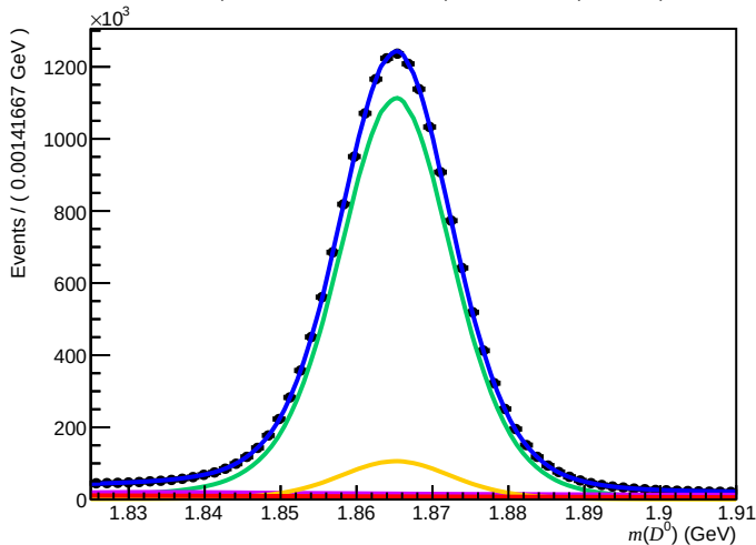
Failed ( 0 < n_{\text{Tracks}} < 200 , 1.7 < \eta < 3.6 , 27000 < p < 60000 )
