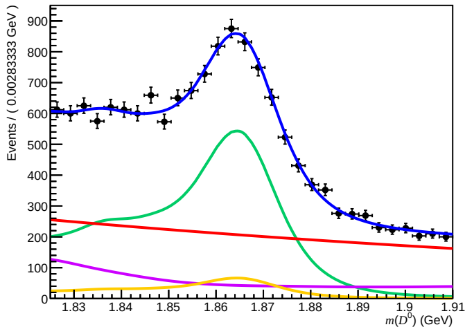
Failed ( 0 < n_{\text{Tracks}} < 200 , 1.7 < \eta < 3.6 , 27000 < p < 60000 )
