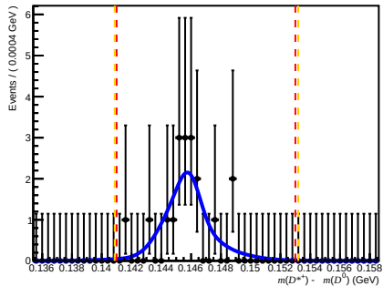
Passed DiF (after RICH1) ( 0 < nTracks < 200 , 3.6 < \eta < 5.0 , 3000 < p < 6000 )
