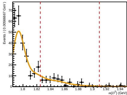
Total ( 0 < nTracks < 200 , 3.6 < \eta < 5.0 , 6000 < p < 10000 )
