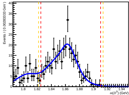
Passed DIF (after RICH1) ( 0 < nTracks < 200 , 3.6 < \eta < 5.0 , 6000 < p < 10000 )
