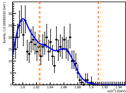
Passed DiF (after RICH1) ( 200 < nTracks < 600 , 1.7 < \eta < 3.6 , 3000 < p < 6000 )
