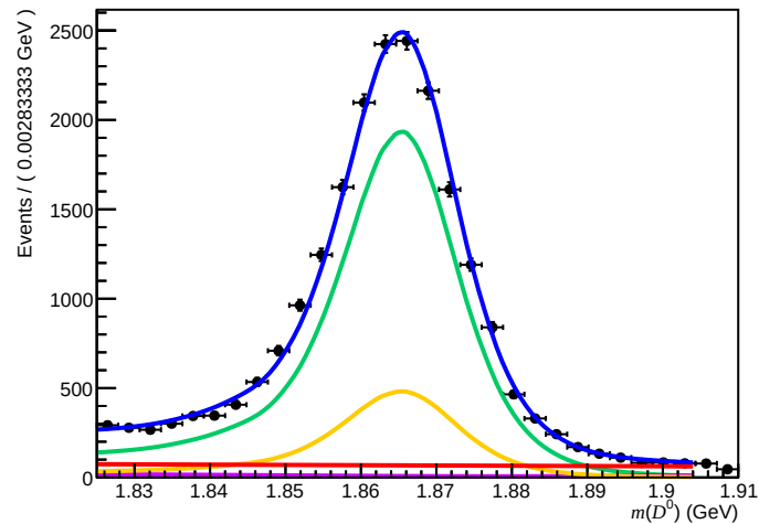
Failed ( 200 < n\text{Tracks} < 600 , 1.7 < \eta < 3.6 , 6000 < p < 10000 )
