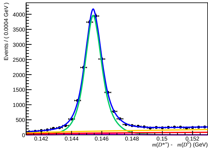
Failed ( 200 < n\text{Tracks} < 600 , 1.7 < \eta < 3.6 , 6000 < p < 10000 )
