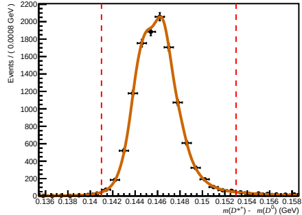
Failed ( 200 < n\text{Tracks} < 600 , 1.7 < \eta < 3.6 , 10000 < p < 15600 )
