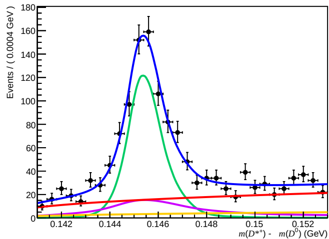
Passed ( 200 < n\text{Tracks} < 600 , 1.7 < \eta < 3.6 , 60000 < p < 100000 )
