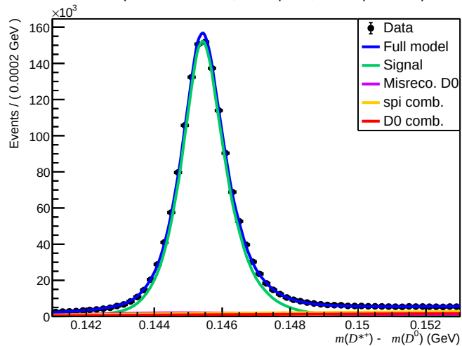
Failed ( 200 < n\text{Tracks} < 600 , 1.7 < \eta < 3.6 , 60000 < p < 100000 )
