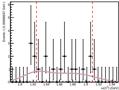
Failed ( 200 < n\text{Tracks} < 600 , 3.6 < \eta < 5.0 , 10000 < p < 15600 )
