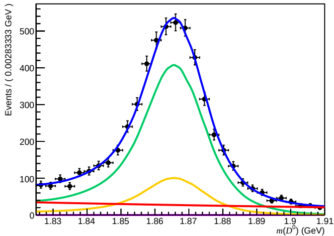
Failed ( 200 < n\text{Tracks} < 600 , 3.6 < \eta < 5.0 , 15600 < p < 27000 )
