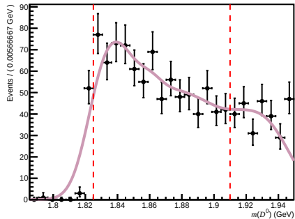
Failed ( 200 < n\text{Tracks} < 600 , 3.6 < \eta < 5.0 , 27000 < p < 60000 )
