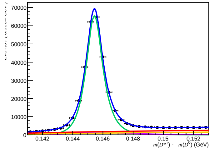
Failed ( 0 < n_{\text{Tracks}} < 200 , 1.7 < \eta < 3.6 , 15600 < p < 27000 )
