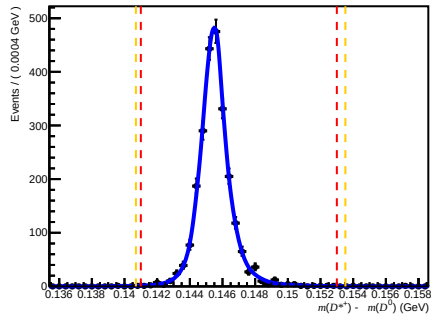
Failed DfF ( 0 < nTracks < 200 , 1.7 < \eta < 3.6 , 60000 < p < 100000 )
