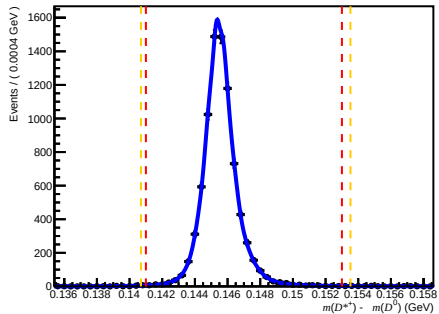
Passed DfF (after RICH1) ( 0 < nTracks < 200 , 1.7 < \eta < 3.6 , 60000 < p < 100000 )
