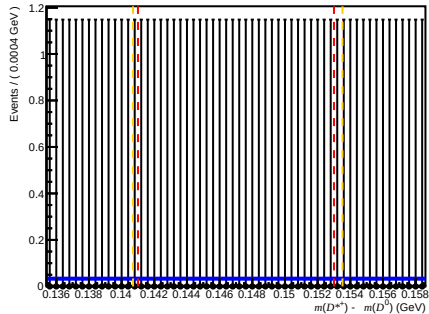
Passed DfF (before RICH1) ( 0 < nTracks < 200 , 1.7 < \eta < 3.6 , 60000 < p < 100000 )
