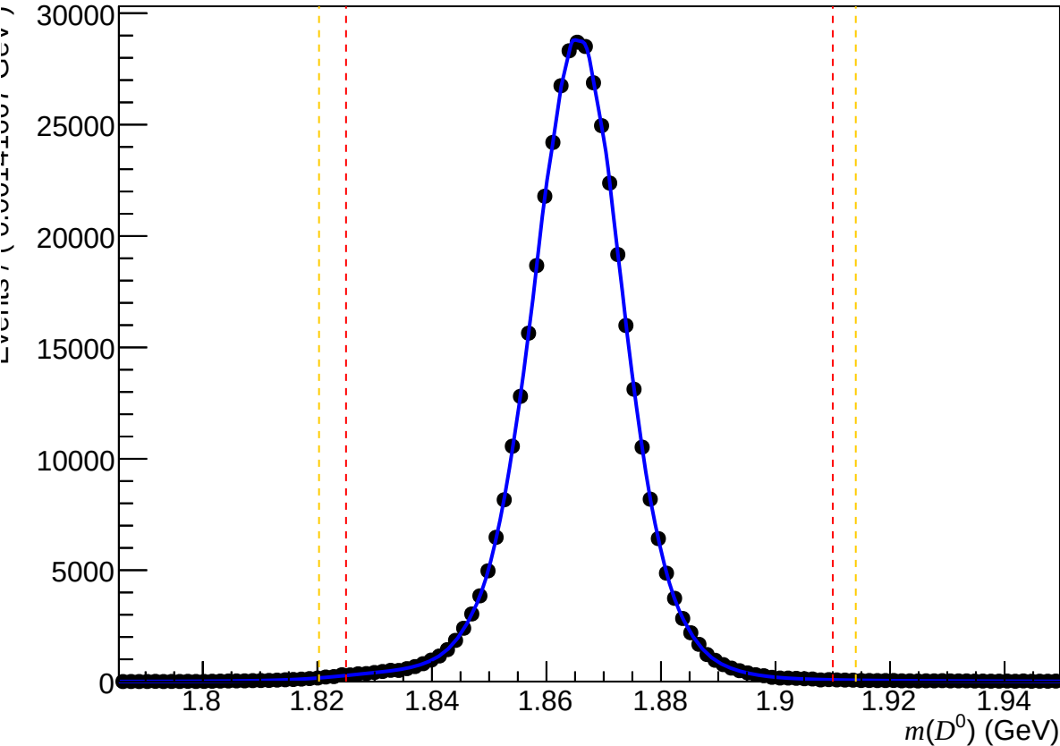
Failed non-DiF ( 0 < nTracks < 200 , 3.6 < \eta < 5.0 , 6000 < p < 10000 )
