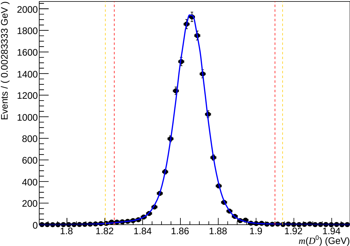
Passed non-DiF ( 0 < nTracks < 200 , 3.6 < \eta < 5.0 , 6000 < p < 10000 )
